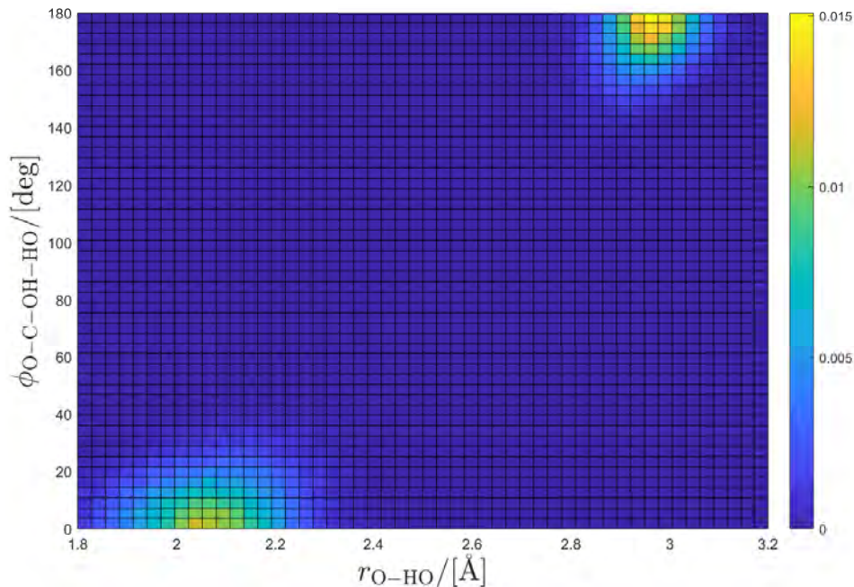
Figure 5.8: The O-C-OH-HO dihedral angle of decanoic acid at various intramolecular O-HO distances in TBAC-dec at 343 K and 1 atm. The various colors describe the probabilities for the combination of the dihedral angle and O-HO distance within each grid cell, according to the color bar on the right-hand side. The data were obtained from snapshots of atomic coordinates from all 5 independent NVT runs (for the last 100 ns to 150 ns).
