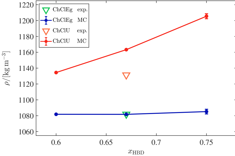
Figure 4.4: Computed liquid densities of ChClEg (at 353 K) and ChClU (at 393 K) as a function of the mole fraction of the HBD component (ethylene glycol or urea) in the liquid phase. The solid lines are drawn to guide the eye. The (extrapolated) experimental data by Yadav and Pandey [181] (for ChClU), and Yadav et al. [36] (for ChClEg) are also shown for comparison.
