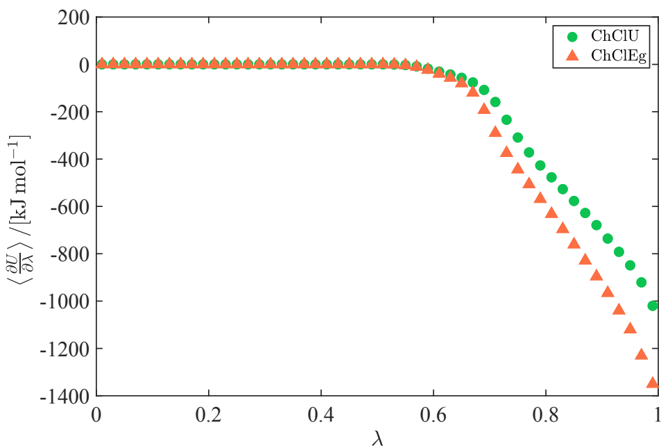
Figure A19: Average values of the derivative of the total energy with respect to \lambda , as a function of \lambda , for choline chloride in ChClU (at 393 K) and ChClEg (at 353 K), from gas phase MC simulations (additional results from chapter 4). The differences between the values of \langle \frac{\partial U}{\partial \lambda} \rangle for choline chloride in ChClEg and ChClU result from the different charge scaling factors used for choline chloride: 0.8 in ChClU, and 0.9 in ChClEg.
