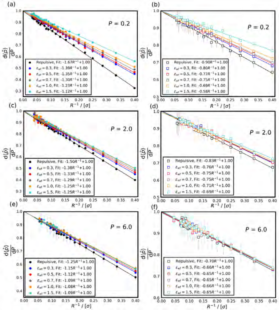
Figure 2.5: The ratio of driving forces, \frac{d(\bar{\rho})}{dP} , is shown as a function of the inverse radius, R^{-1} , of box 2 at P = 0.2, 2.0 , and 6.0 for the cylindrical and slit pore cases with repulsive and attractive wall potentials. In subfigures (a), (c), and (e), \frac{d(\bar{\rho})}{dP} is shown for cylindrical pores at differential pressure P = 0.2, 2.0 , and 6.0 , respectively. In subfigures (b), (d), and (f), \frac{d(\bar{\rho})}{dP} is shown for slit pores at differential pressures P = 0.2, 2.0 , and 6.0 , respectively. The simulation results are shown with symbols, while the lines are fits to the data points. The equation used for the fitting is AR^{-1} + B , where A and B are constants. The results for the cylindrical pore are shown with closed circles and for the slit pores with open rectangles. The colors denote the different wall potential used in box 2, repulsive wall potential (black), \epsilon_{wf} = 0.3 (blue), \epsilon_{wf} = 0.5 (red), \epsilon_{wf} = 0.7 (gray), \epsilon_{wf} = 1.0 (orange), and \epsilon_{wf} = 1.5 (cyan). The temperature of both boxes is set to T = 2 . The average densities of box 1 are \rho \approx 0.10, 0.58 , and 0.8 at P = 0.2, 2.0 , and 6.0 , respectively.
