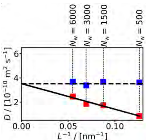
Figure 7.1: The computed self-diffusion coefficients of \beta -CD as a function of the inverse of the simulation box length at T = 298.15 K and P = 1 bar. The symbols in red and blue colors indicate the calculated self-diffusion coefficients without and with using the YH correction [436], respectively. N_w denotes the number of water molecules used in the simulation. For modelling the \beta -CD and water the q4md-CD [369] and TIP4P2005 [295] force fields were used, respectively. The maximum statistical error in the computed self-diffusion coefficients is 10%. The error bars are smaller than the symbol size.
